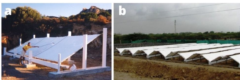
Figure 2. some large radiative dew condensers. (a) In Ajaccio (Corsica island, France). [Source: Photo D. Beysens]. (b) In Kothara (North-West India) [Source: Photo G. Sharan]
